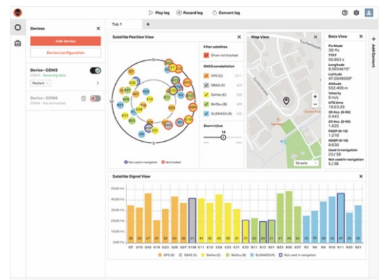
u-center 2
