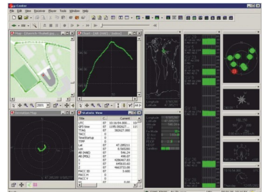
u-center
